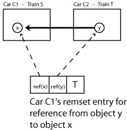
Figure 6.1 - An Example Remset Entry
