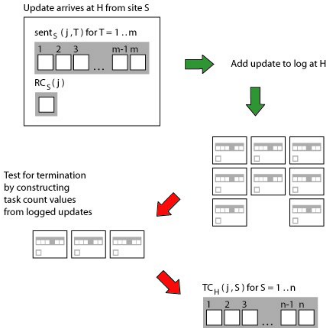
Figure 4.2 - Standalone Updates and Termination Detection
