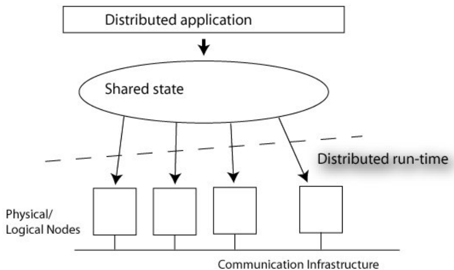
Figure 1.1 - Shared Application State in a Distributed Run-Time
