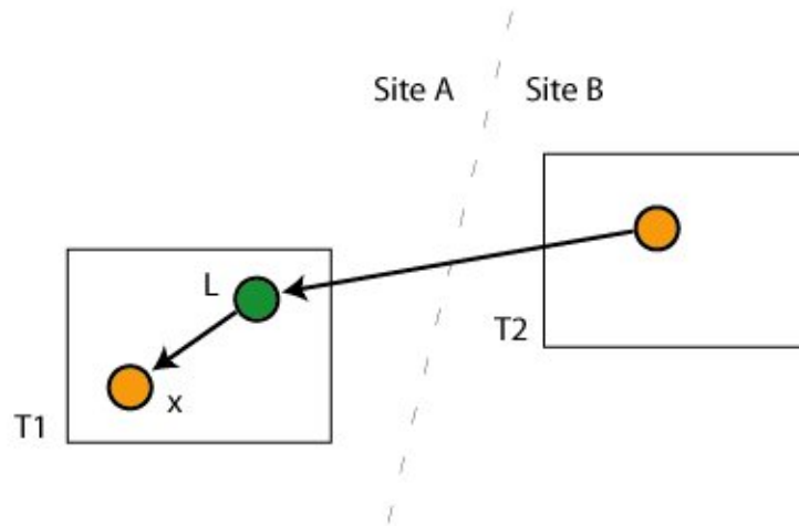
Figure 6.9 - Remote Dereference
