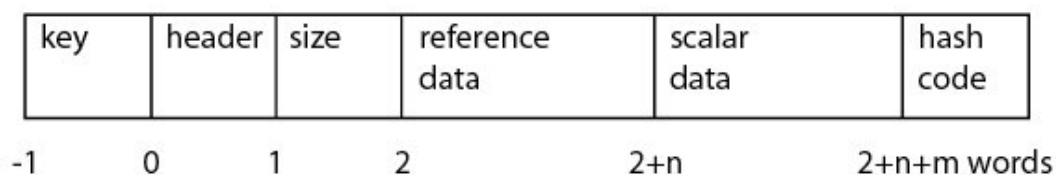
Figure 3.4 - The Uniform Object Format
