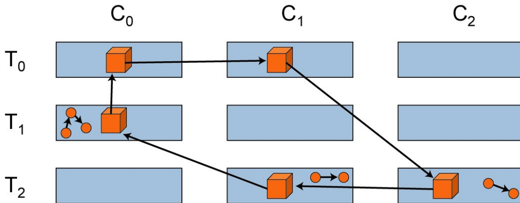
Figure 6.2 - A Garbage Cycle held in Three Trains
