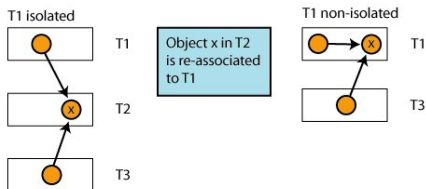
Figure 6.7 - The Unwanted Relative Problem
