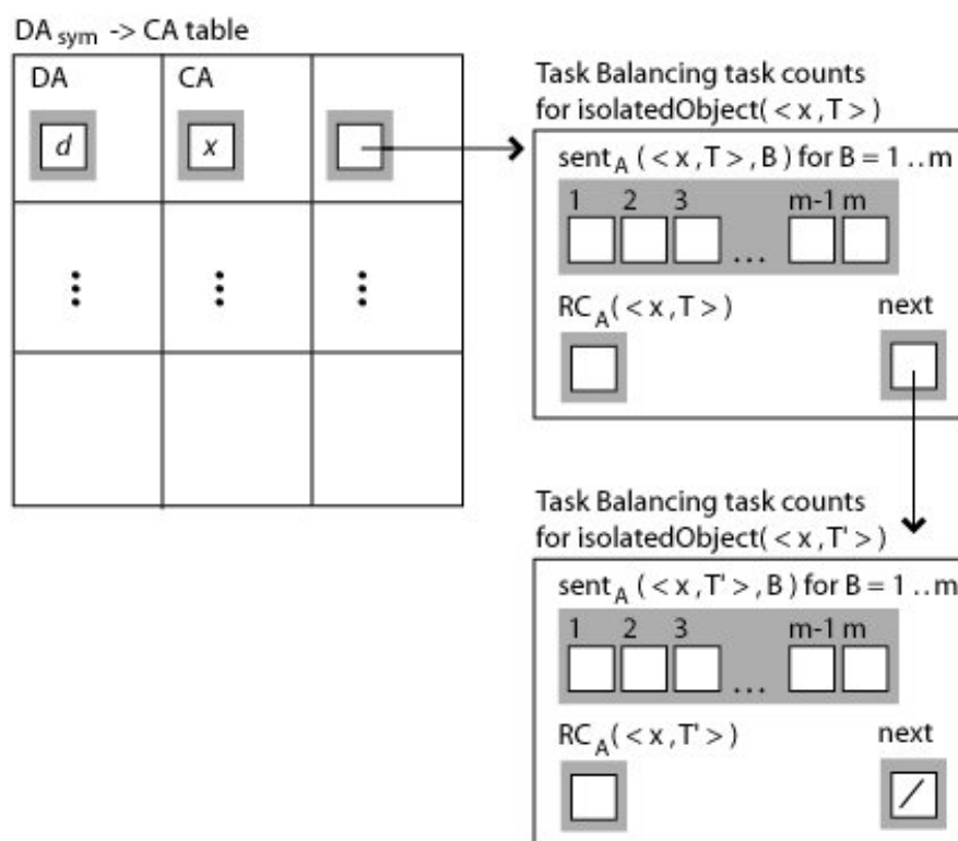
Figure 7.5 - The \text{DA}_{\text{sym}} \rightarrow \text{CA} Table with TB task Count Structures
