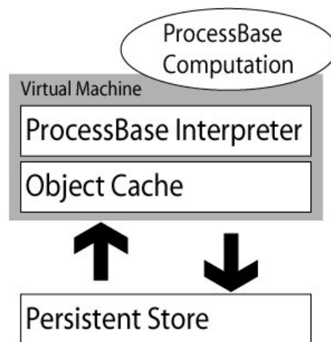
Figure 3.1 - The ProcessBase Runtime Architecture
