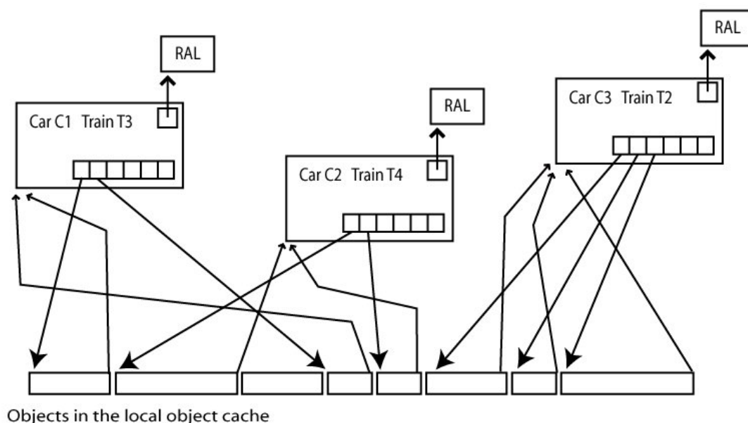
Figure 7.1 - Associating Objects with Cars
