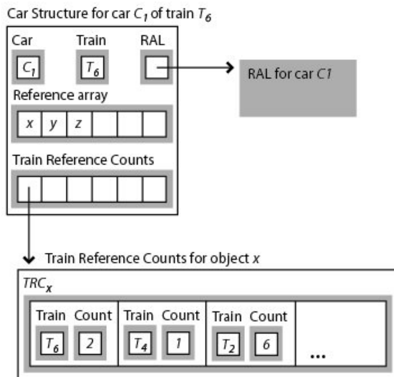
Figure 7.3 - The Car Data Structure
