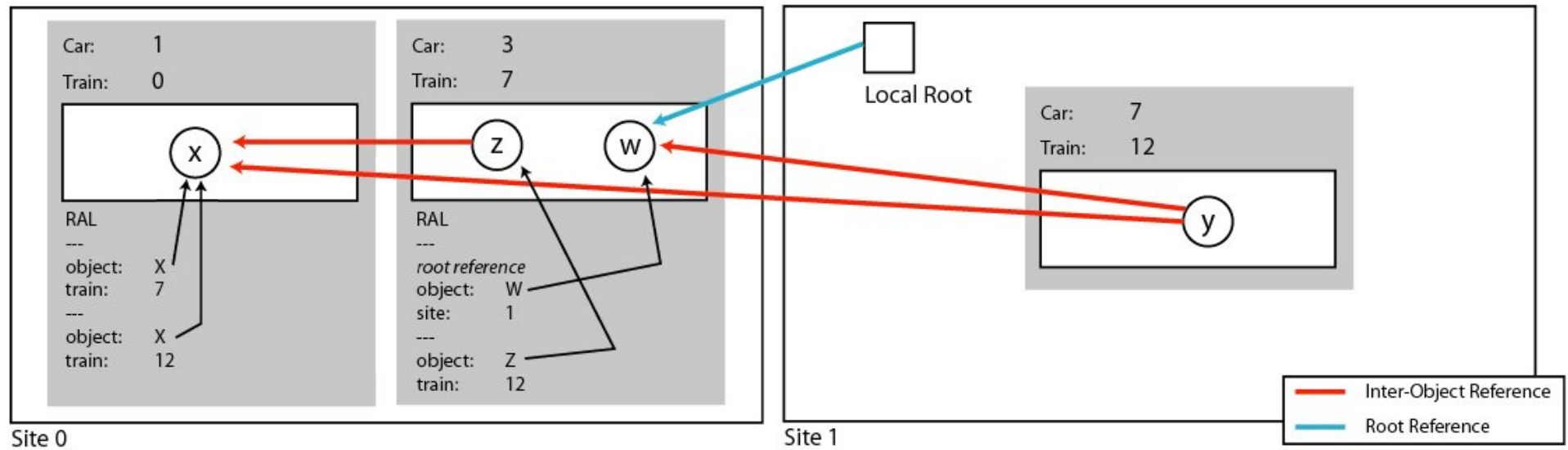
Figure 6.8 - Example RAL Entries
