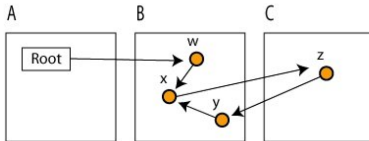
Figure 2.3 - Rudalics's Counter Example
