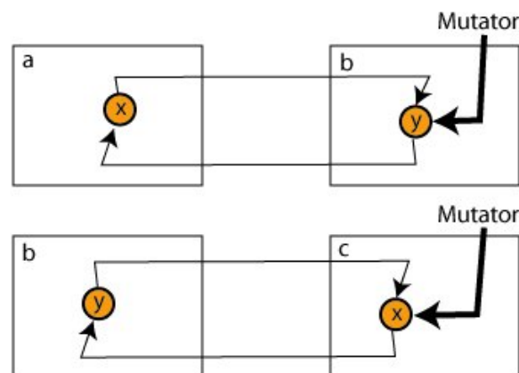
Figure 6.6 - The Zero-Progress Problem
