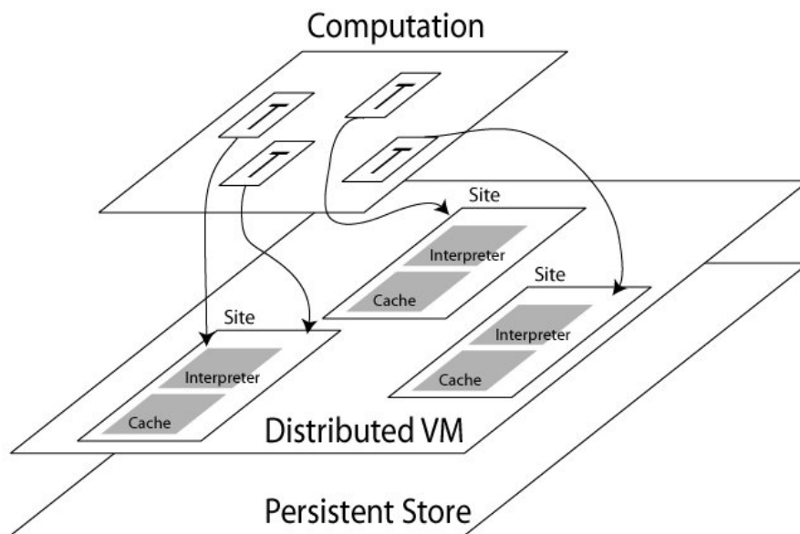
Figure 3.3 - ProcessBase Computational Model
