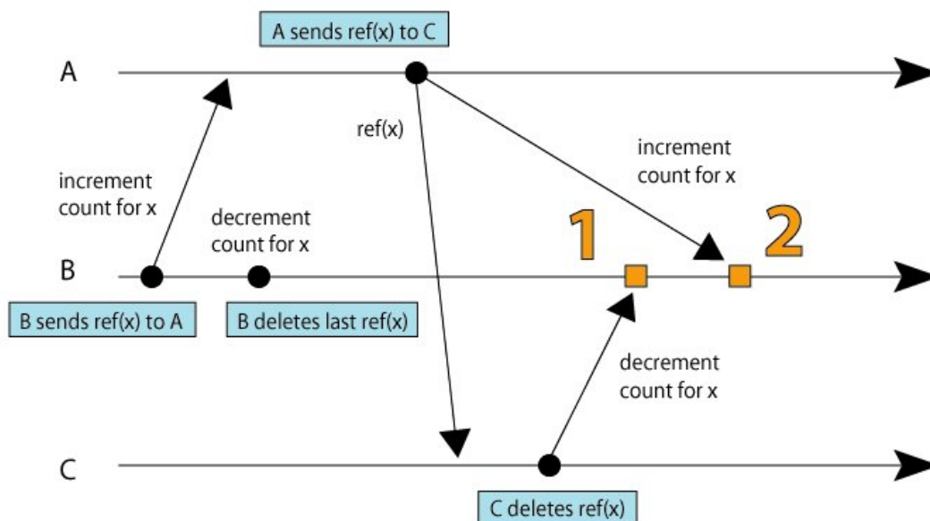
Figure 2.1 - Distributed Reference Counting Race Condition
