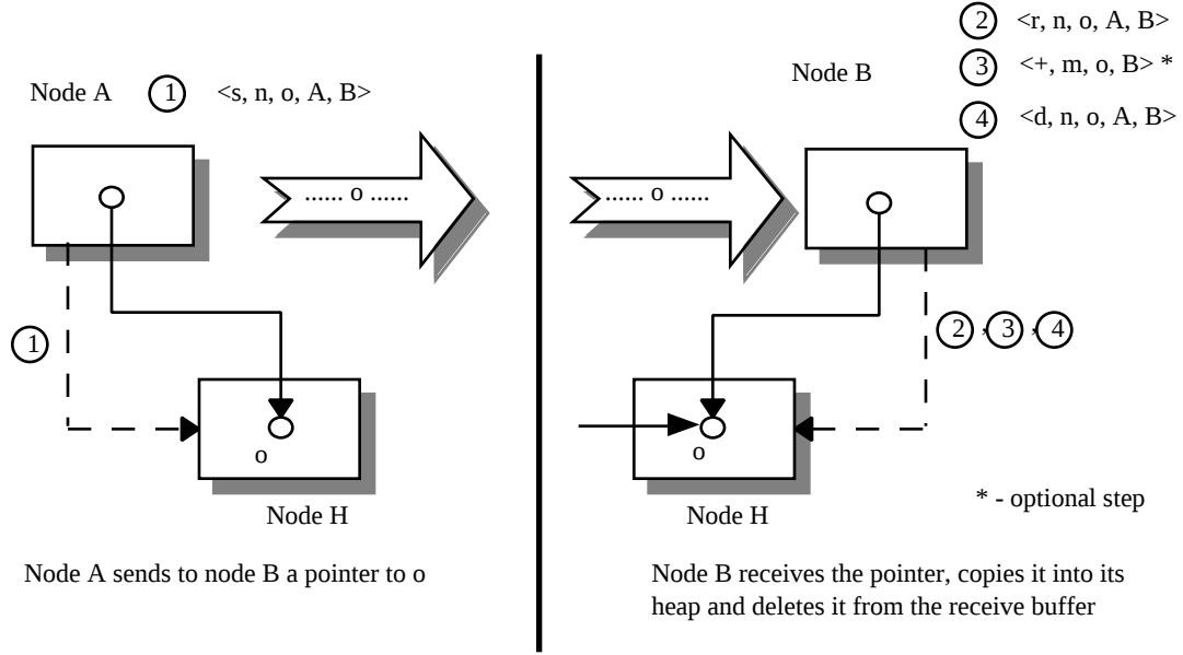
Figure 2: Node A Sends to Node B a Pointer to o
