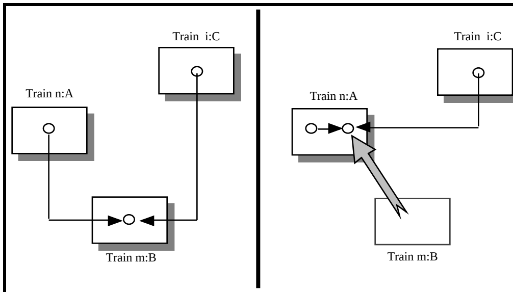
Figure 5: The “Unwanted Relative” Problem
