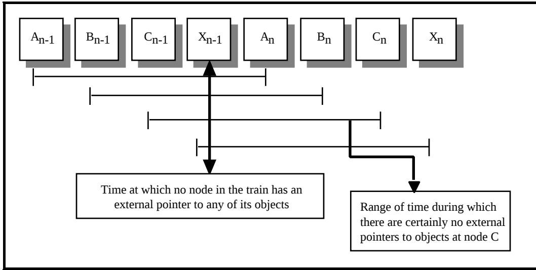
Figure 4: Illustration of Correctness of the Train Reclamation Algorithm
