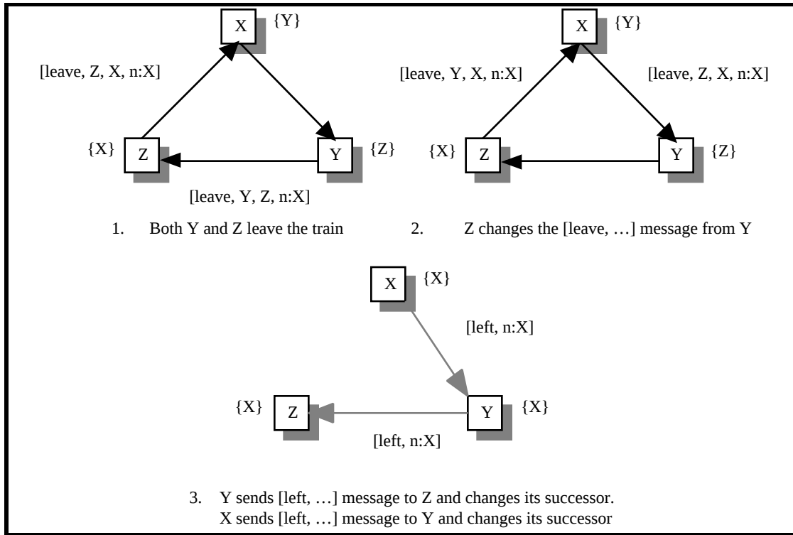
Figure 3: Two Nodes Leave a Train Ring at the Same Time
