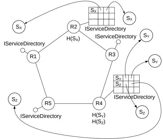
Figure 5. Example system state
