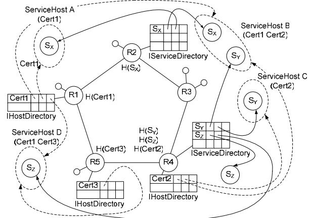
Figure 8. Service Hosts and service instances
