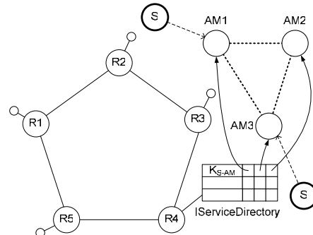
Figure 10. Peered Autonomic Managers
